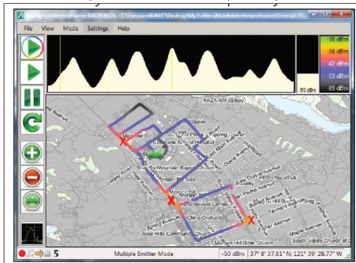
Figure 3. Multi-Emitter mode
